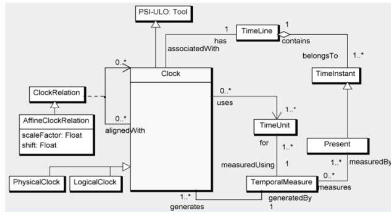
(b) A UML class diagram formalizing the natural language definition of a Clock (Figure 2a). The corresponding OWL code for a Clock is omitted.
